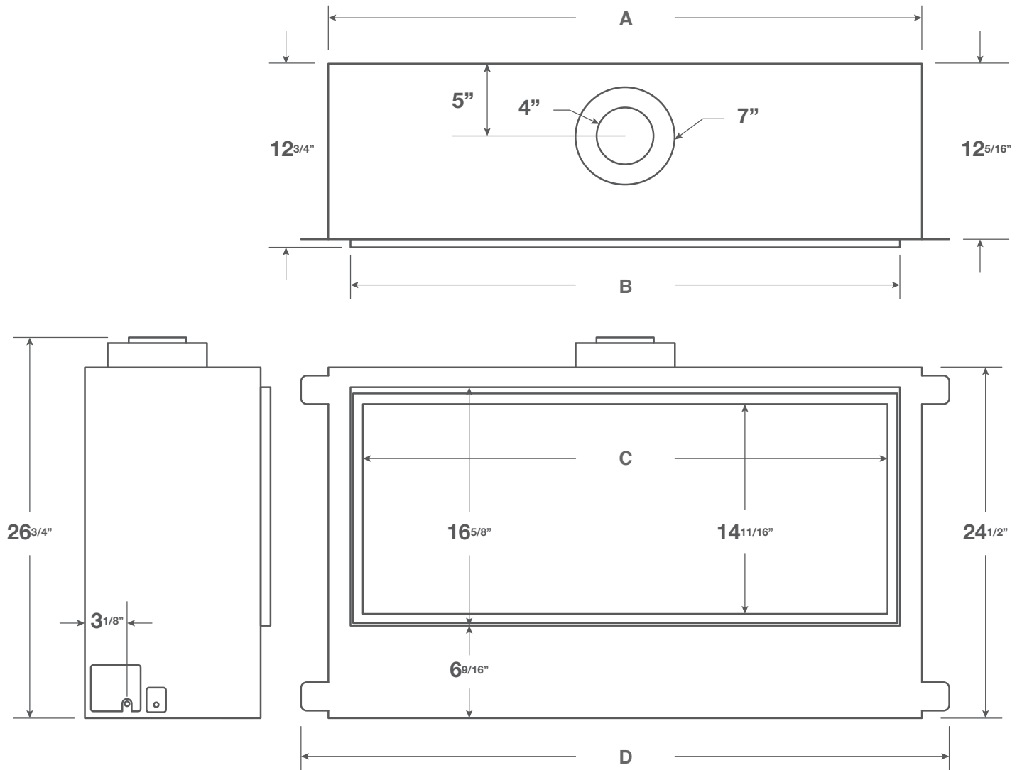
Figure 2. DelRay Fireplace dimensions (Tolerance \pm 1/8" ).
