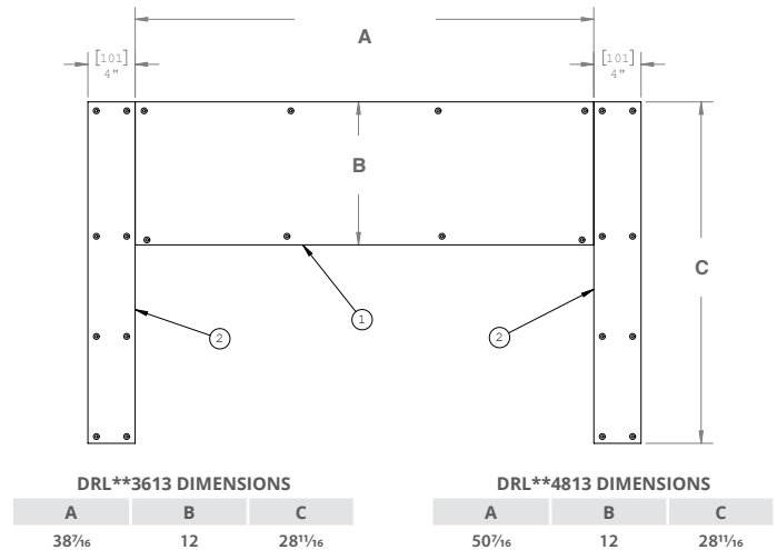
Figure 28. Supplied non-combustible cement board dimensions
