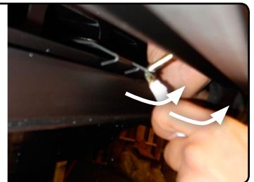
Figure 21.e Lift the latch upward
