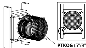
Figure 10.f Installing a PTO termination heat guard.
