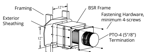
Figure 10.c Installing a PTO termination with the BSR frame.
