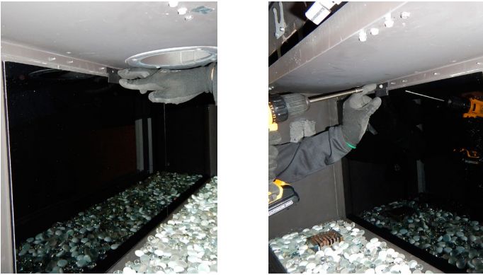
Figure 26.d Secure panel
