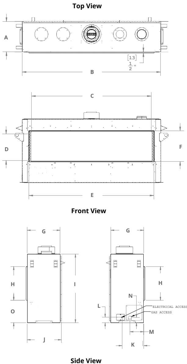
Figure 2. DL6315, D6315 Fireplace dimensions (Tolerance \pm 1/8" ).
