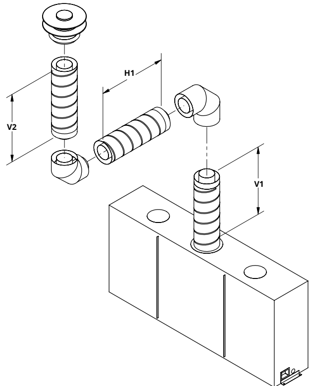
Figure 8.b Vertical Termination - 2 Elbows
